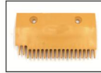
A-FLY ID: AF-LG40132G Part ID: DSA2000168-R Size: 163*95mm*19T Hole distance :90 Material: plastic Color: yellow
