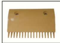
A-FLY ID: AF-LG40134C Part ID: 2L0081316 Size: 145*90mm*16T Hole distance : 90 Material: plastic Color: yellow
