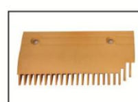
A-FLY ID: AF-FT140031B Part ID: 0129CAE001 Size: 203*100*22T Hole distance : 130 Material: plastic Color: yellow
