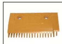
A-FLY ID: AF-HI20003B Part ID: H2200124 9905003N Size: 164*90*19T Hole distance :90 Material: plastic Color: yellow
