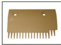
A-FLY ID: AF-LG40132A Part ID: DSA2000168-L Size: 146*95mm*17T Hole distance :90 Material: plastic Color: yellow
