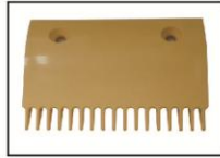
A-FLY ID: AF-LG40132C Part ID: DSA2000169-M Size: 142*95mm*17T Hole distance :90 Material: plastic Color: yellow
