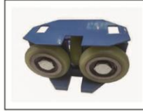
A-FLY ID:GS-046 wheel diameter:76mm Suitable for Elevator
