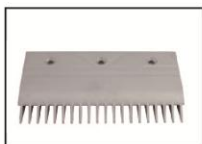
A-FLY ID:AF-MI10048B Part ID: J651058B203 Size: 181*94*20T Hole distance : Material: aluminum Color: Silver/natural
