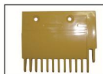
A-FLY ID:AF-MI10867B Part ID:YS125B688 Size: 117*97*13T Hole distance :54 Material: plastic Color: yellow
