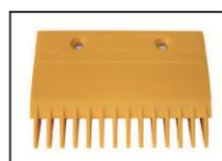
A-FLY ID: AF-MI10047A Part ID:9905007N YS017B313 Size: 127*94*14T Hole distance :64 Material: plastic Color: yellow
