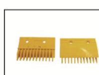
A-FLY ID: AF-FT140062B Part ID:X129V1 Size:105*80*12T Hole distance : Material: plastic Color: yellow
