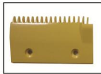
A-FLY ID: AF-LG40134A Part ID: 2L0081317 Size: 160*90mm*17T Hole distance : 90 Material: plastic Color: yellow
