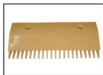
A-FLY ID: AF-LG40404C Part ID: DSA2001489A-M Size: 198*94mm*22T Hole distance : 120 Material: plastic Color: yellow
