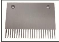
A-FLY ID: AF-OT80509A Part ID: XAA453J1 Size: 193.2*145.3*23T Hole distance : 142 Material: aluminum Color: Silver/natural
