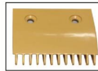
A-FLY ID: AF-LG40134B Part ID: 2L0081319 Size: 108*90mm*12T Hole distance : 60 Material: plastic Color: yellow
