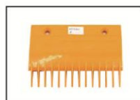
A-FLY ID: AF-MI10048C Part ID:YS013B578 Size: 127*94*14T Hole distance :80 Material: plastic Color: yellow
